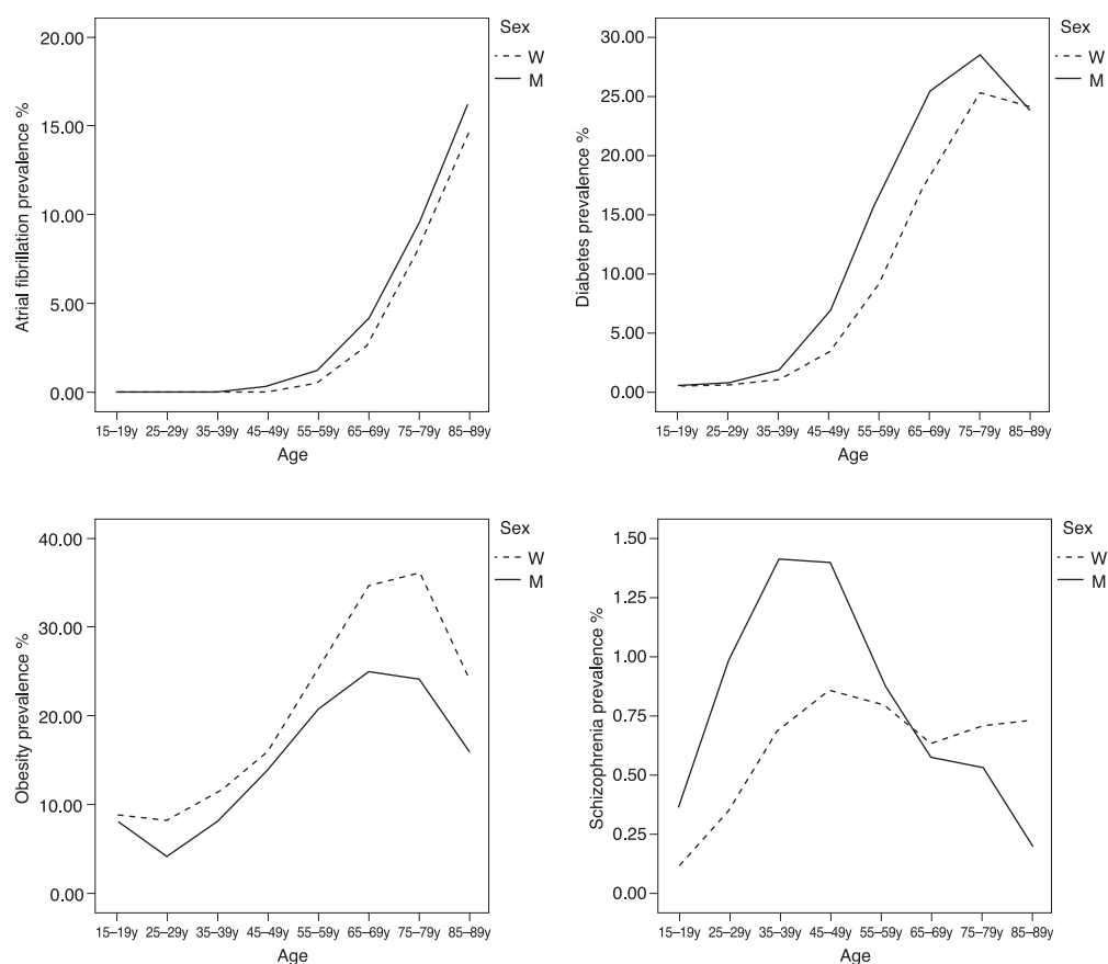
Figure 2 RQS reference prevalences by age and sex
