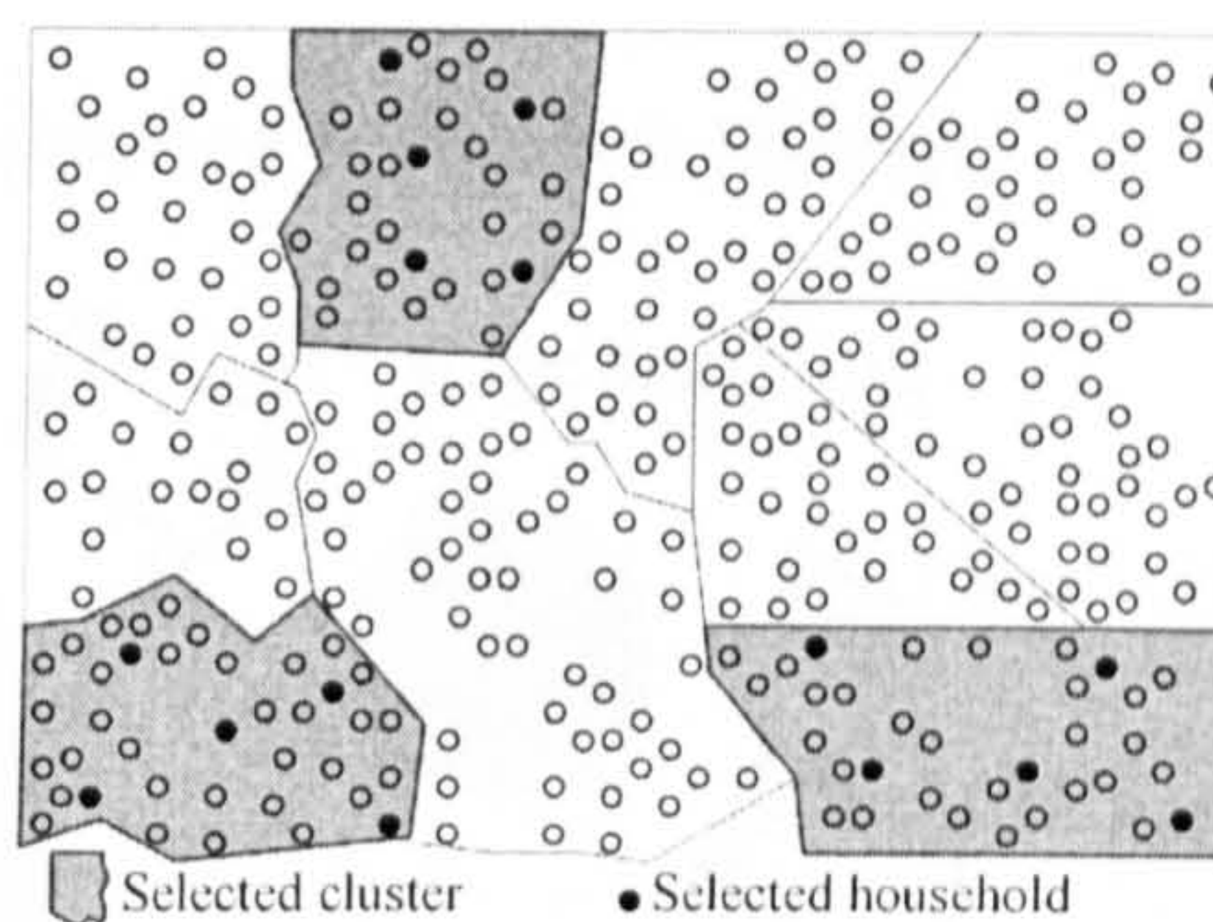
Figure 5.2: Example of two stage sampling
