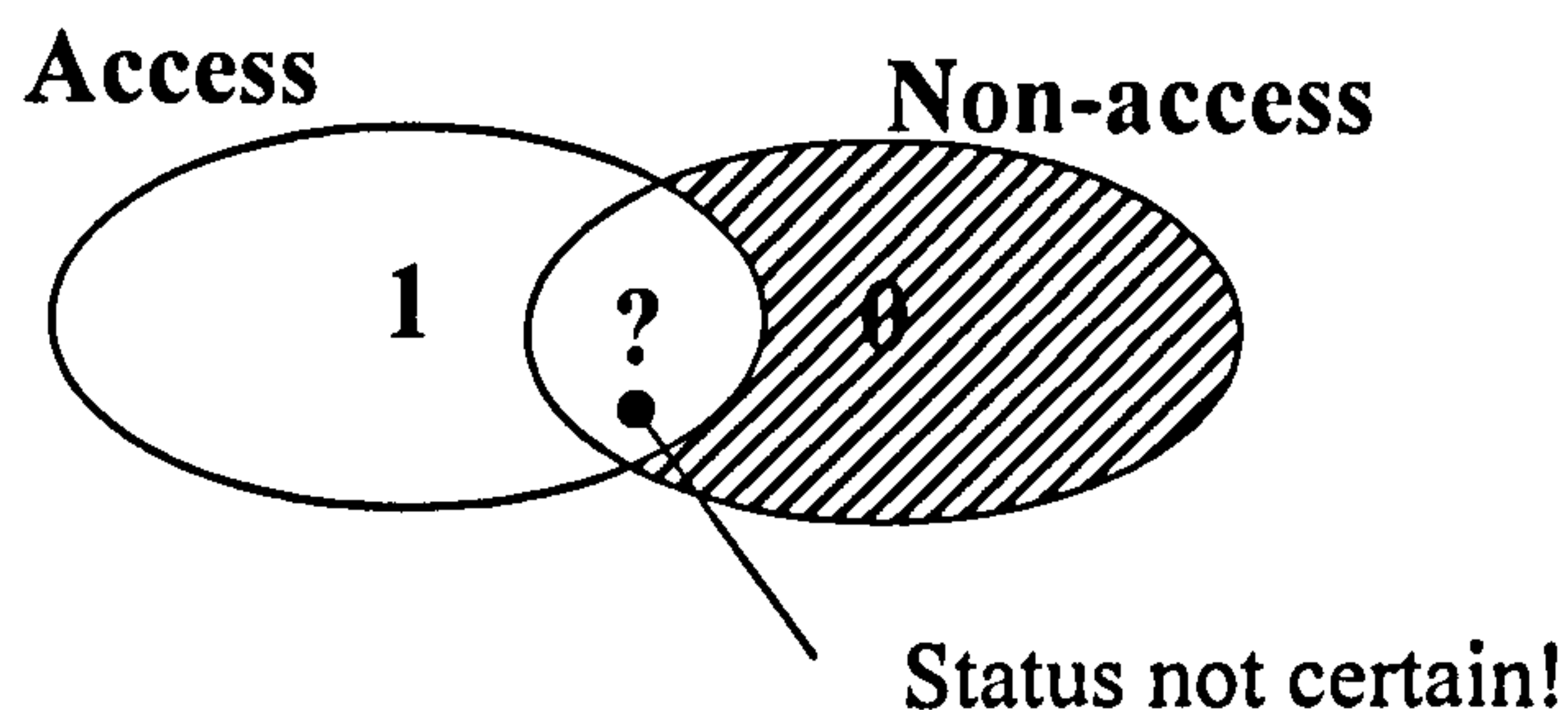
Figure 9: Area in Venn diagram measured by survey.
