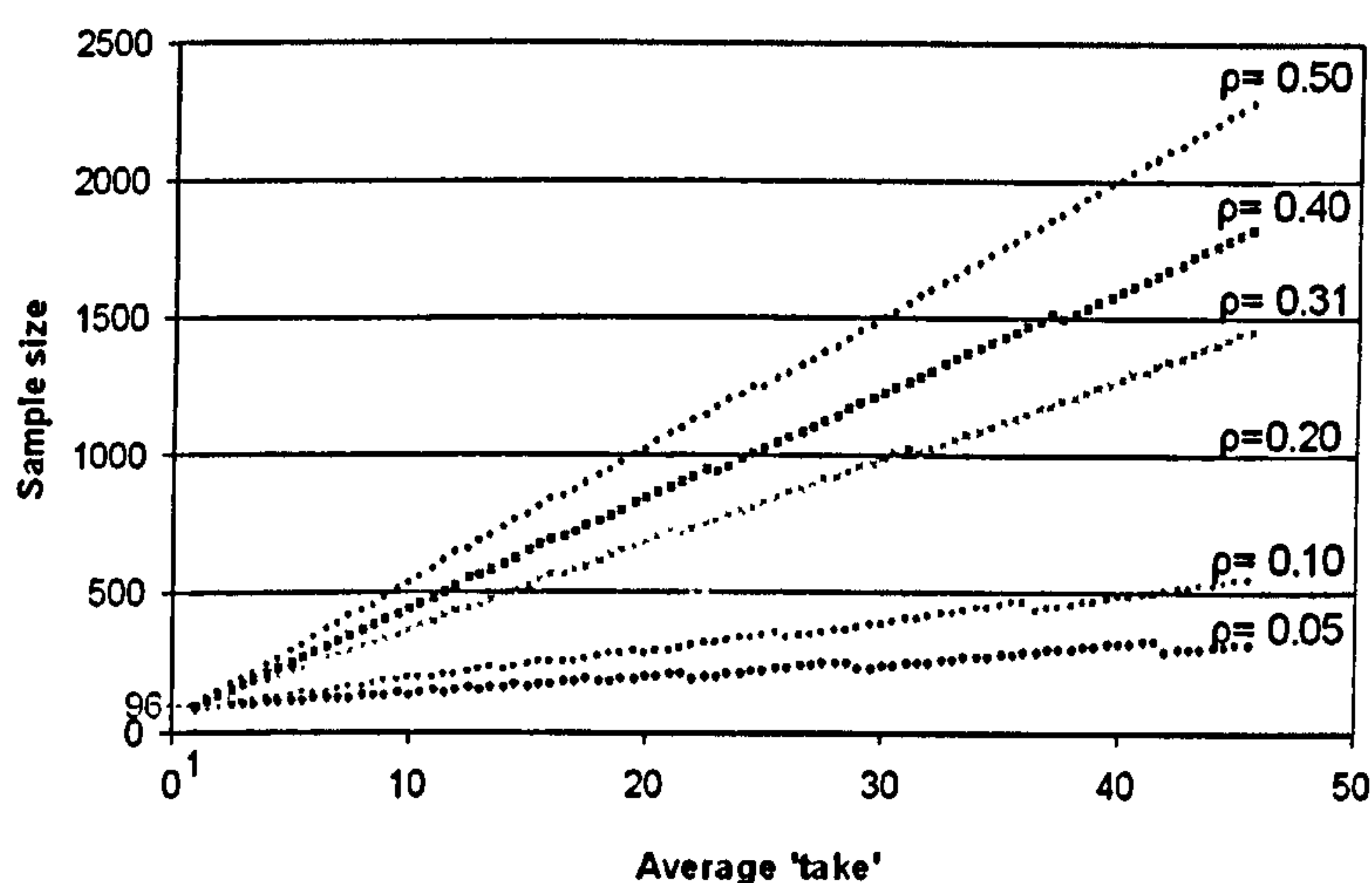
Graph 5.2: Sample size in function of the take for different values of \rho
