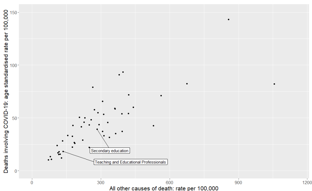
Figure 1 Scatterplot of mortality rate (per 100 000) for COVID-19 and all other causes of death for men, using ageadjusted mortality rates between 9 March and 28 December 2020 from the Office for National Statistics. Unlabelled data points represent occupational groups in online supplemental table S4. Pearson's correlation coefficient=0.78, p=1.4\times 10^{-11} .
