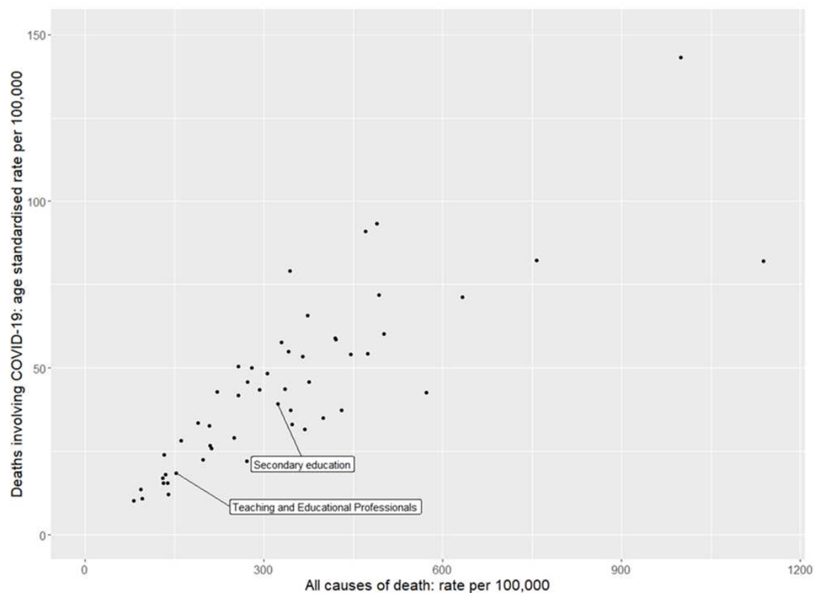
Figure S1 – Scatterplot of mortality rate (per 100,000) for Covid19 and all-cause mortality for men, between 9th March and 28th December 2020
