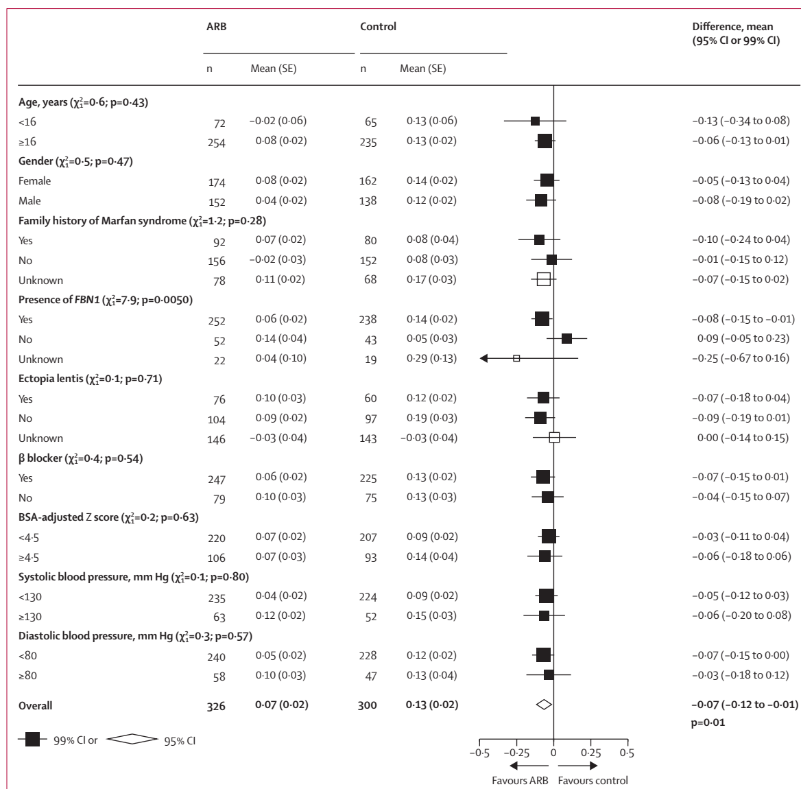
Figure 2: Annual rate of change of BSA-adjusted aortic root dimension Z score at the sinuses of Valsalva, by subgroups (ARB vs control) ARB=angiotensin receptor blocker. BSA=body surface area.
