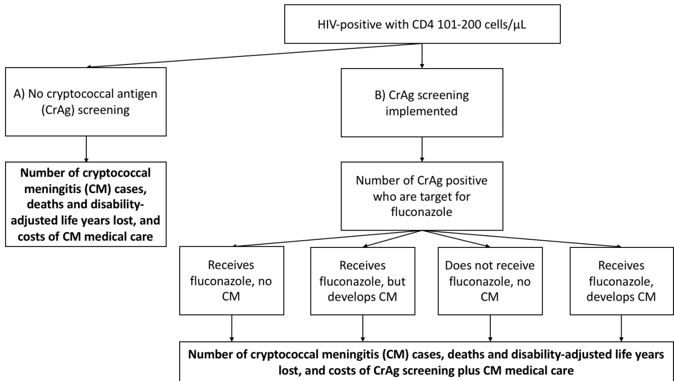
Figure 1. Overview of model. The model compares cryptococcal meningitis cases, related deaths and disability-adjusted life years lost, and costs between no cryptococcal antigen screening and implementation of screening at a CD4 count of 101–200 cells/ \mu\text{L} .
