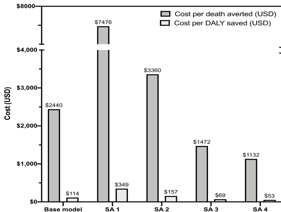
Figure 2. Estimated costs per death averted and disability-adjusted life year saved under base model and sensitivity analyses. DALY = disability-adjusted life year; SA = sensitivity analysis; USD = United States dollar.
