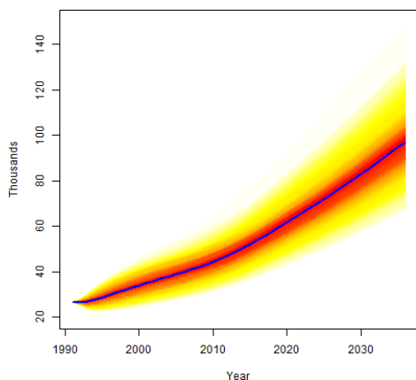
Figure 2 Fan plot of the estimated number of people with dementia. The weighted average of all simulations is shown in Blue. Colours depict percentiles of the distribution of the number of cases of dementia from the 100 simulations with the lowest calibration error.
