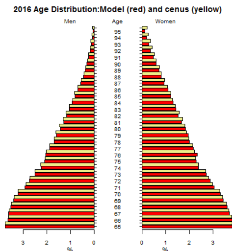
Figure 1 Population age distribution for 2016 for the simulation with the lowest error. Simulation estimates are shown in red and the observed census data are shown in yellow.
