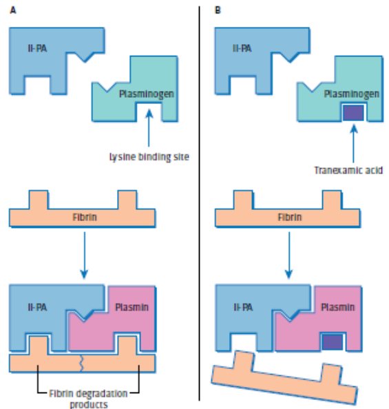
Fig 1 | A Normal fibrinolysis. B: Fibrinolysis inhibited by tranexamic acid. Plasmin binds to fibrin via lysine binding sites and then splits fibrin into fibrin degradation products. Tranexamic acid is a molecular analogue of lysine that inhibits fibrinolysis by reducing the binding of plasmin to fibrin
