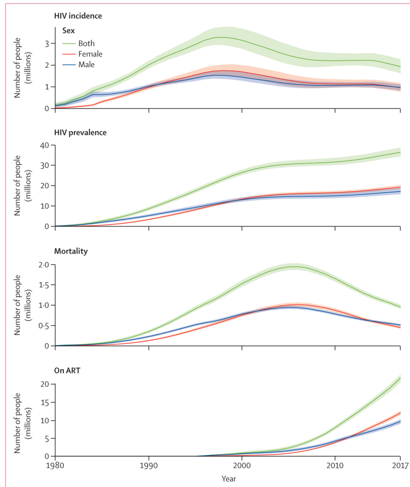
Figure 1: Global HIV incidence, prevalence, mortality, and people on ART, by sex, for all ages, 1980–2017
