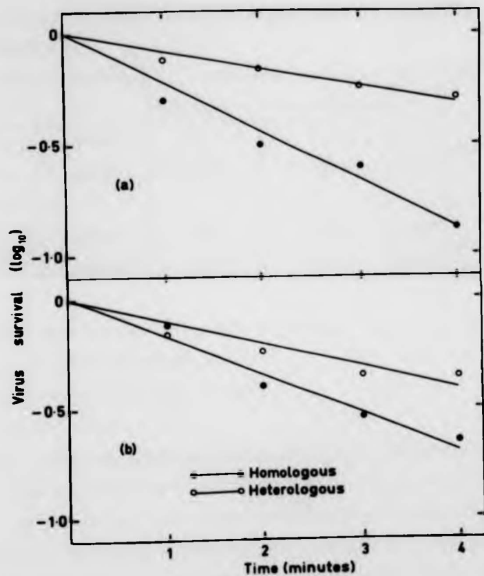
Figure 3.3. Kinetic curves of neutralisation of (a) A6003 virus and (b) A6900 virus by homologous and heterologous antisera.
