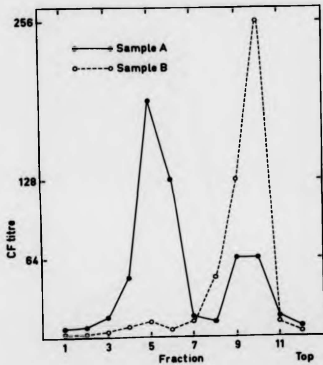
Figure 2.5. Comparison of the CF activities of fractions from sucrose density gradients for the preparation of natural 12S antigen from Sample A and VIA antigen from Sample B.
