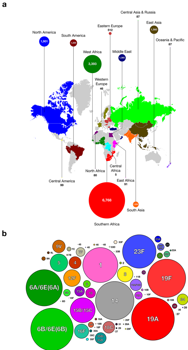
Fig. 1. (a) World map showing the global distribution of the samples in the study dataset. (b) Bubble plot showing the 66 serotypes included in the dataset (the area of each circle is proportional to the number of samples).
