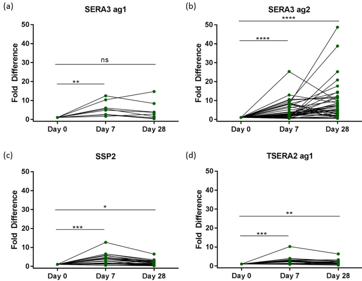
Figure 5. Serial fold increase in antibody reactivity for each antigen following treatment of knowlesi malaria. (a) SERA3 ag1, (b) SERA3 ag2, (c) SSP2 and (d) TSERA2 ag1. Asterisks indicate level of significance, ns denotes non-significant values ( p \leq 0.0001 ****; p \leq 0.001 ***; p \leq 0.01 **; p \leq 0.05 * and p > 0.05 ns).
