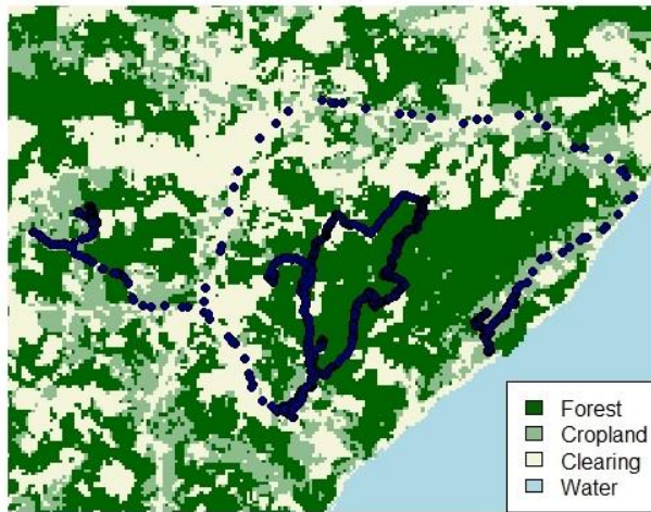
Figure 6.7. a. GPS tracks from single individual over classified land use map and, b. utilisation distribution calculated for this individual using BRB
