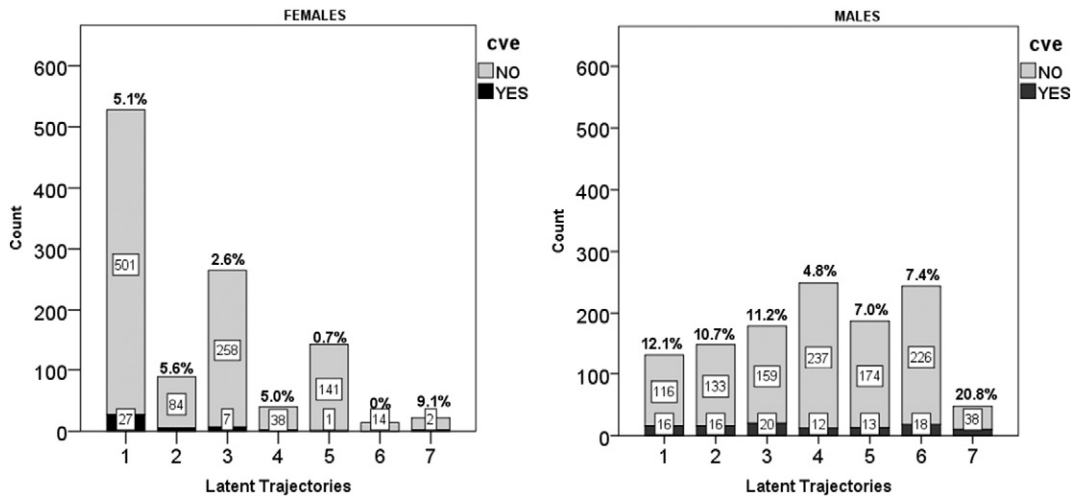
Fig. 3. Absolute counts of CVE and CVE-free subjects assigned to the extracted latent trajectories. Crude CVE prevalence per trajectory (%) is given.
