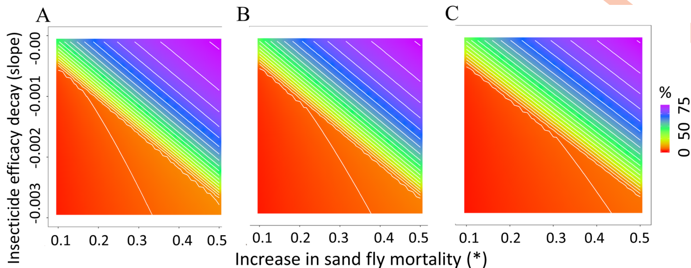
Fig 3. Reduction of human incidence of L. infantum infection. Scenario of mass application of systemic insecticides to dogs. Dog coverage: 80% (A), 70% (B) and 60% (C). Insecticide efficacy (horizontal axis) is represented by the increase in sand fly mortality caused by the insecticide ( \mu_T(0) ). Decay in the insecticide efficacy occurs at a constant rate per day (vertical axis). Contour curves mark 5% changes in human incidence.
