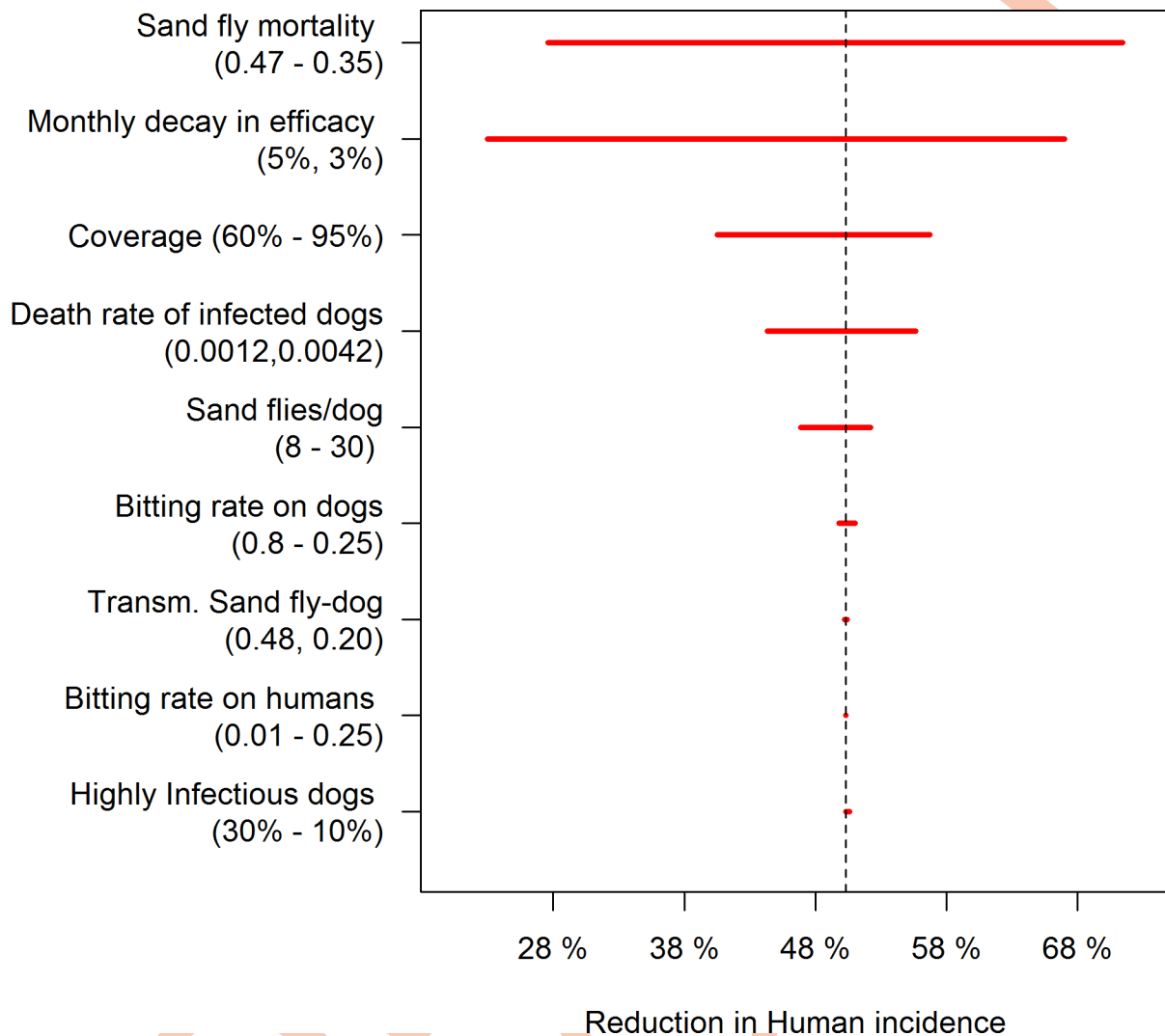
Fig 4. Tornado plot showing the sensitivity of different parameters on the reduction in human incidence of L. infantum infection in the model.
