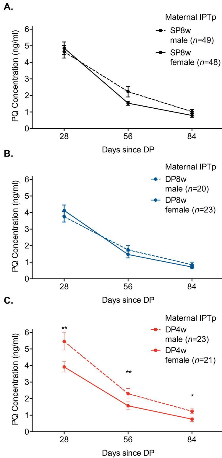
Fig 4. Mean PQ levels measured 28, 56, and 84 days posttreatment among children whose mothers were randomized to IPTp-SP8w (A), IPTp-DP8w (B), and IPTp-DP4w (C). Marginal estimates obtained using generalized estimating observations with log link and robust standard errors, accounting for repeated measurements in
