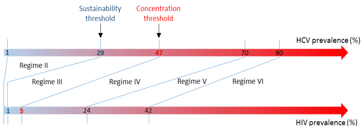
Figure 6.3. Summary of the overlapping epidemiology of HCV and HIV infections among people who inject drugs. The figures displays the different dynamical regimes and the HCV thresholds for sustainable and concentrated HIV epidemics. (Note: Regime 1, where the prevalence of both infections is less than 1%, is not displayed on the graph)
