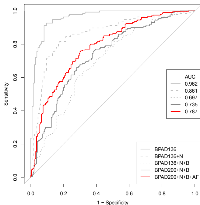
Figure 2. ROC curves were generated from SVM classifiers utilizing 10 features selected by greedy backward feature elimination in a LTOCV approach. Averages were plotted across five iterations of SVM classifiers implemented to randomly break ties resulting from the greedy backward feature elimination procedure. The benchmark to assess these modifications was a non-nested, non-balanced training data set of 136 BPAs and 136 non-BPAs annotated with 122 features from 19 protein annotation tools (BPAD136) [20]. Subsequent modifications were added in a stepwise fashion and included: a nested cross-validation approach (BPAD136+N), balanced selection of non-BPAs for predicted subcellular localization (BPAD136+N+B), increased size of training data (BPAD200+N+B), and additional features (525 total) derived from an increased number of protein annotation tools (BPAD200+N+B+AF).
