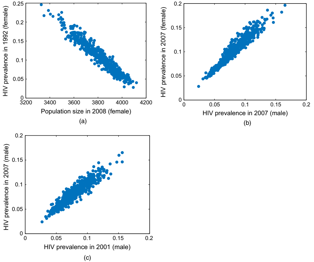
Fig. 8. Scatter plots of mean output values from simulator runs at wave 7: the large correlation between outputs is an indication of the way that the simulator models the HIV transmission across sexes and across time (see the text)
