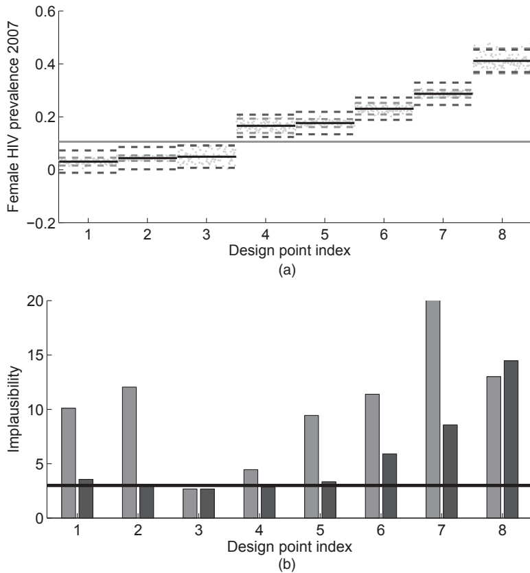
Fig. 2. Improvements due to the emulated variance method: (a) 100 simulator evaluations in eight different design points ( \bullet ), their mean (—) and \pm 2 standard deviations calculated with V_{s,90} (---) or with the actual variance calculated by the 100 repetitions at each design point (—) (—, mean of the empirical data); (b) simplified form of the implausibility calculated with V_{s,90} (■) or with the actual variance (■) (—, implausibility cut-off)
