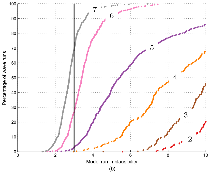
Fig. 3. Cumulative distribution function of simulator run implausibility I_{\mathcal{R}}(\mathbf{x}) , by wave (each curve represents the percentage of each wave's simulator runs with an I_{\mathcal{R}}(\mathbf{x}) less than the value indicated by the horizontal axis; the numbers on the curves indicate the wave number): (a) fixed variance; (b) emulated variance
