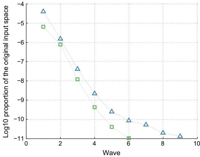
Fig. 4. Proportion of the samples drawn at random in the original simulator input space, that are non-implausible after k waves of history matching (the emulated variance methodology proposed achieved the same reduction of non-implausible space in three fewer waves): \square , emulated variance; \triangle , fixed variance
