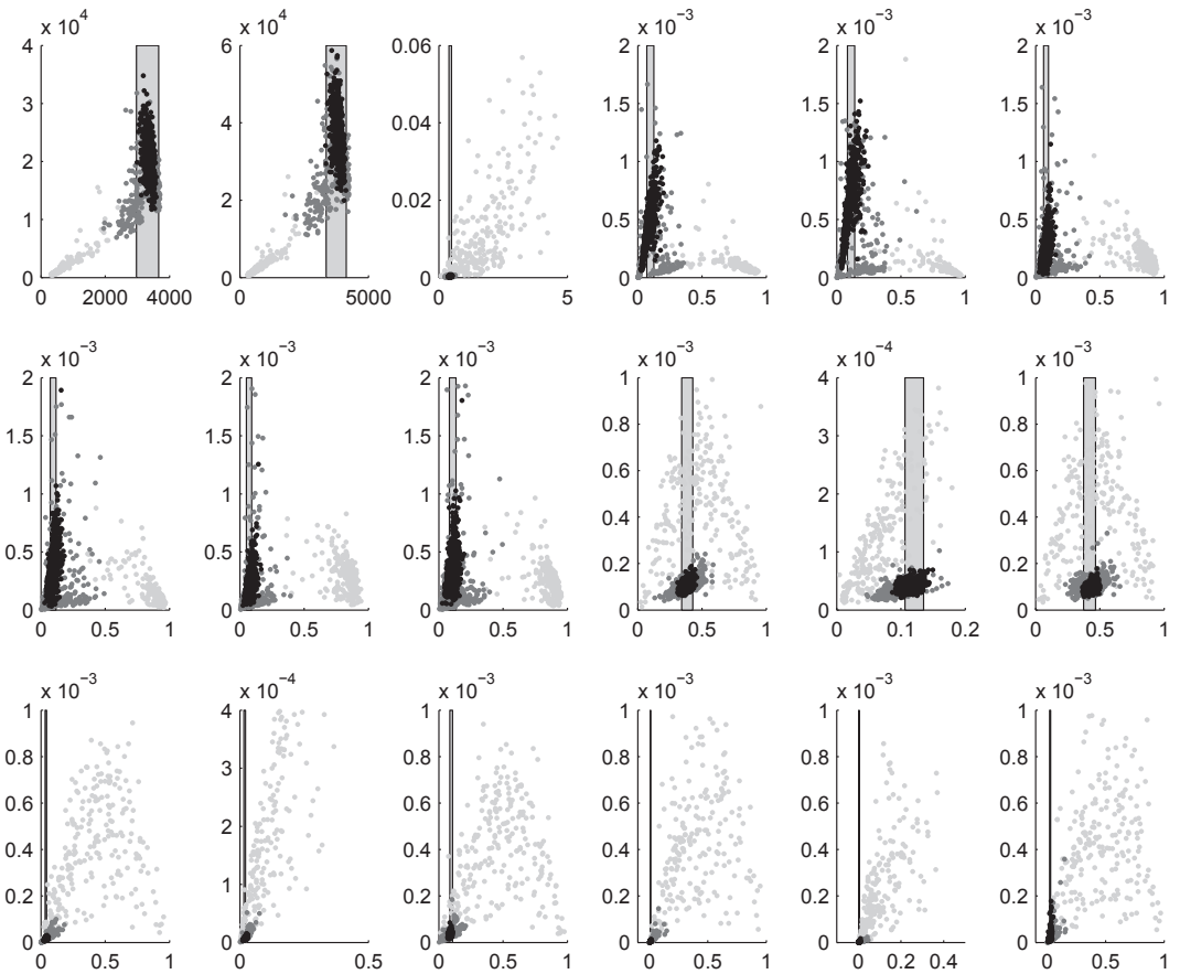
Fig. 7. Scatter plots of the simulator’s mean output (horizontal axis) against its variance (vertical axis) for waves 1 (•), 4 (◦) and 7 (◐); the 18 outputs are arranged first from left to right and then from top to bottom; the vertical patches in each panel show the empirical data on the mean outputs with \pm 2 standard deviations derived from the observation error and model discrepancy at wave 6
