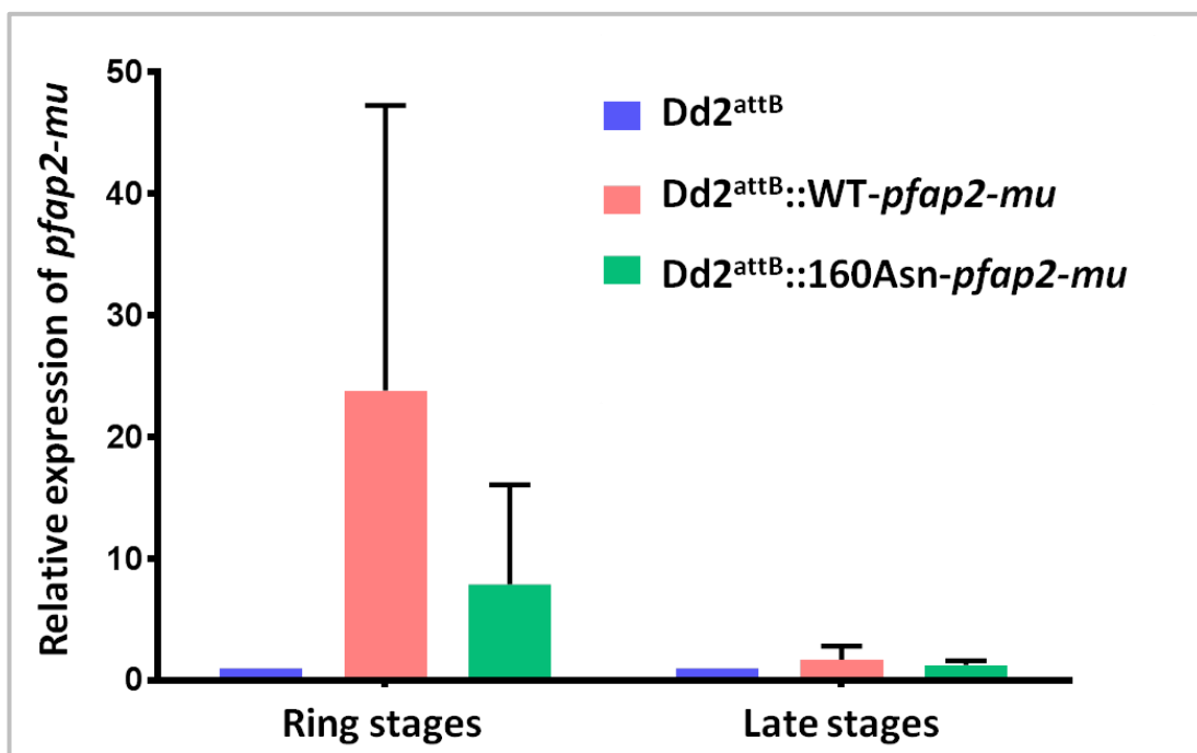
Figure 2. Expression levels of pfap2-mu transcripts on ring and late stage (trophozoites and schizonts) cultures of Dd2 attB , Dd2 attB ::WT- pfap2-mu and Dd2 attB ::160Asn- pfap2-mu lines. Mean mRNA expression level of pfap2-mu in Dd2 attB and transfected lines from RT-qPCR analysis. The expression of pfap2-mu was normalized to the mRNA level of PgMET. Error bars indicate standard deviations.
