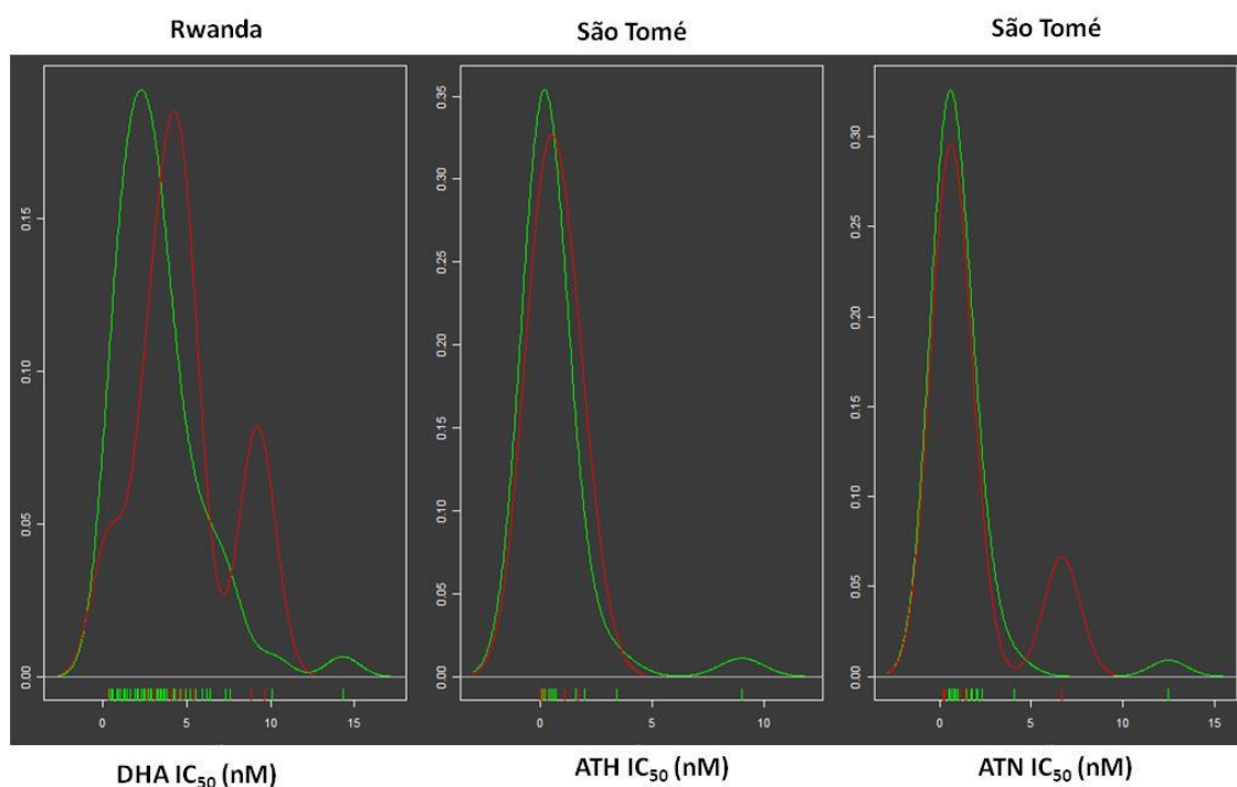
Figure 7: Density function curves for the WT (N160 pfap2-mu ) (in green) and MUT (160S pfap2-mu ) samples (in red). The ticks below the curves illustrate the measured IC_{50} values for each sample. DHA: dihydroartemisinin; ATN: artesunate; ATH: artemether.
