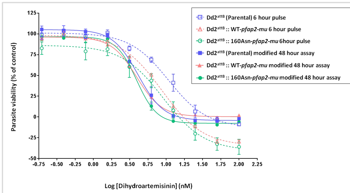
Figure 4. Dose response curves of the Dd2^{attB} (Parental), Dd2^{attB} :: WT-pfap2-mu and Dd2^{attB} :: 160Asn-pfap2-mu transfectants to Dihydroartemisinin. The drug sensitivity of the parasites was assessed using a modified 48 hour assay (solid line) and 6 hour pulse assay (dashed line). Each point represents the mean of two independent experiments, with two replicates for each experiment. The error bars indicate \pm standard errors of the means. Best-fit curves were generated by Prism v6.04. The X axis indicates the increasing concentration of dihydroartemisinin and the Y axis indicates the parasite viability.
