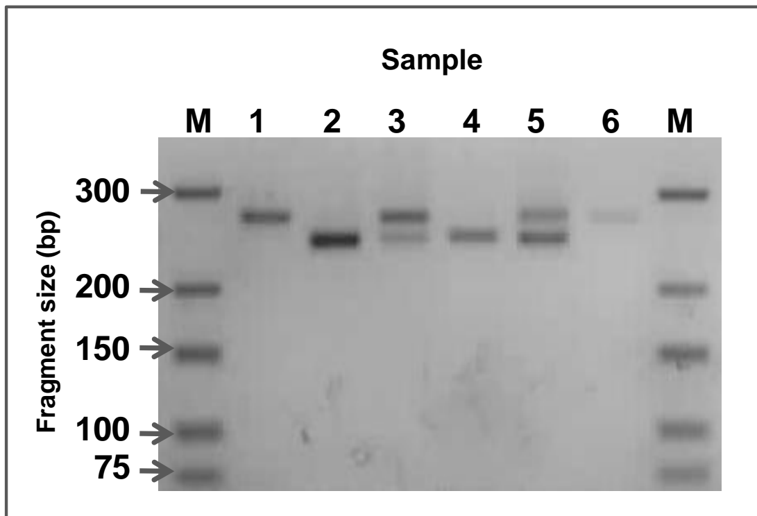
Figure 2. Typical results of the Pfap2-mu gene PIRA-PCR results. M: molecular weight marker. Lanes 1 and 6: Pfap2-mu 160N variants; lanes 2 and 4 Pfap2-mu 160S variants; lanes 3 and 5: mixture of genotypes. Samples were run in 3% agarose gels stained with ethidium bromide
