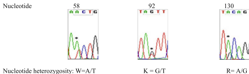
Fig. 1. Inter-discrete typing unit (DTU) diversity in the trypanostigote small surface antigen (TSSA) gene sequences. (A) Nucleotide polymorphisms within and between DTUs of the TSSA gene fragment across the panel of Trypanosoma cruzi reference strains. (B) Nucleotide heterozygosity in the CL Brener strain is represented by the degenerate symbols W, K and R. GenBank™ accession numbers refer to sequences derived in this study. Previous nomenclature for TcII–VI[IIa–e] is shown in brackets.
