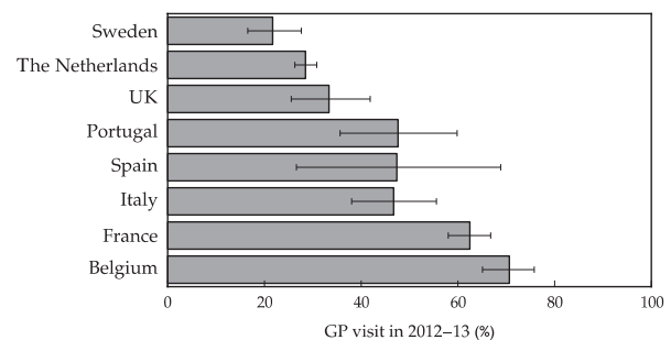
FIG. 2. Visits to general practitioners (GPs) reported by Influenzanet users.
