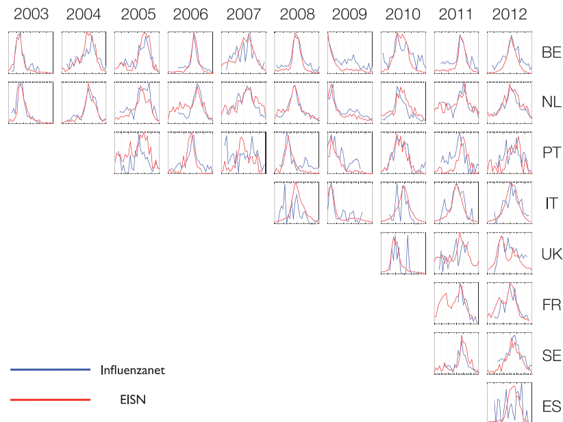
FIG. 1. Weekly incidence data (influenza-like illness cases/100 000) for eight countries from 2003–2004 to 2012–2013. All the curves are rescaled on the maximum. Vertical lines correspond to months from November to May for each year. EISN, European Influenza Surveillance Network; BE, Belgium; NL, The Netherlands; PT, Portugal; IT, Italy; FR, France; SE, Sweden; ES, Spain; UK, United Kingdom.
