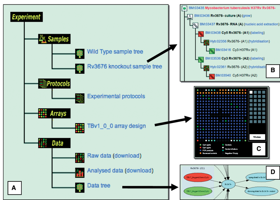
Figure 1. BμG@Sbase stores all experimental data and displays an overview schematic on each experiment page (A), sample descriptions are displayed as interactive trees (B), an interactive viewer provides access to array design information (C), raw and analysed data is linked through a network of transformations (D).
