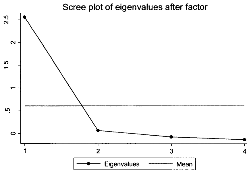
Figure 5: Scree plot for the factor analysis for the structural quality index
