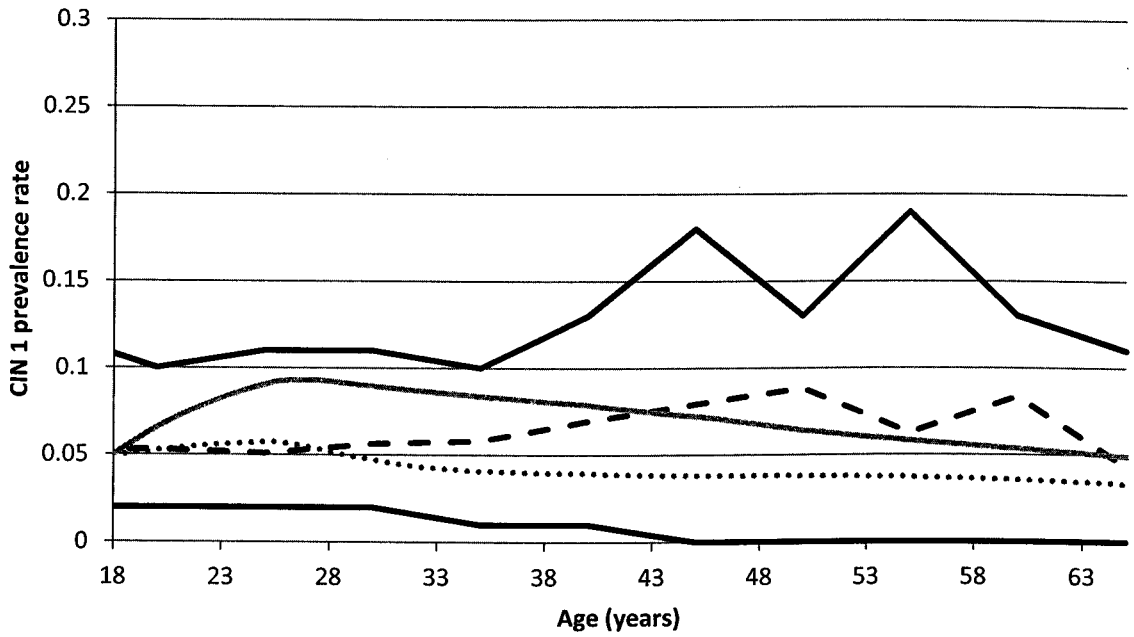
Figure A.1: Age-specific CIN 1 prevalence rate (calibration result)
