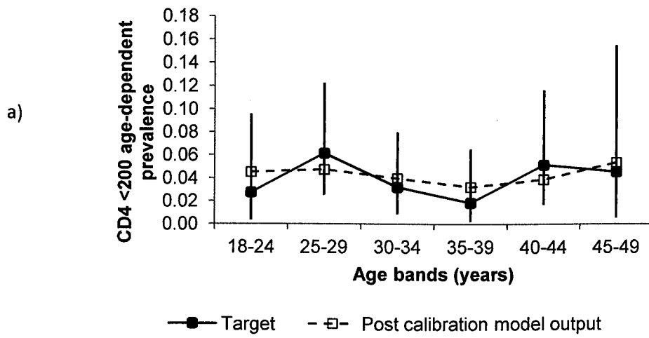
Figure 6.1 a,b,c: Calibration results
