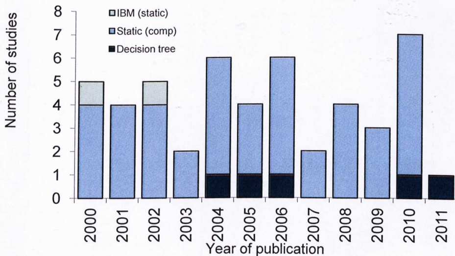
Figure 3.2: Modelling methods used in screening studies
