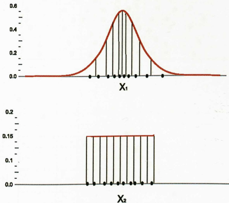
Figure 4.3: Examples of probability density functions associated with parameters X_1 and X_2
