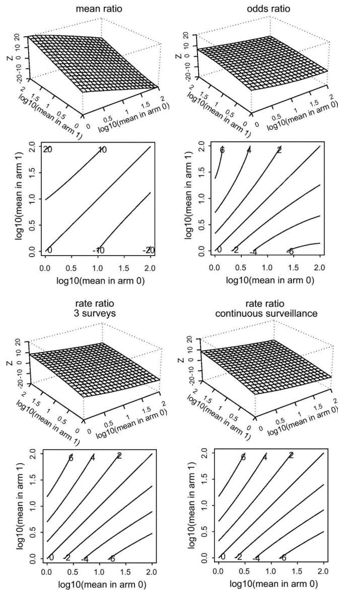
Fig. 2. Surface and contour plots of Z statistics from four candidate effect measures. The horizontal axes in the surface plots, and both axes in the contour plots, show possible values of mean infection intensity (number of parasites seen per person) in the two arms ('0' and '1') of a trial with 100 people per arm and a fixed value of 0.5 for negative binomial dispersion parameter ( k ). The vertical axis in the surface plot, and the contour values in the contour plot, show Z statistics: the expected value of the test statistic divided by its standard error. A Z statistic of 2 (or -2 ) corresponds to a two-sided p value of 0.05, and Z = 4 corresponds to p = 0.00006 . Comparing the effect measures, a higher Z value for the same means indicates greater statistical power. For any combination of mean infection intensity, the ratio of means has the highest absolute value of Z , and so is the most powerful effect measure, followed by the rate ratio. The ratio of means achieves Z values more than 20, while the others do not reach Z = 10 . Whether the rate estimation is based on three examination rounds, or continuous surveillance, makes little difference, as indicated by comparing their Z values for any given combination of mean infection intensities in the two arms. Finally, the odds ratio
