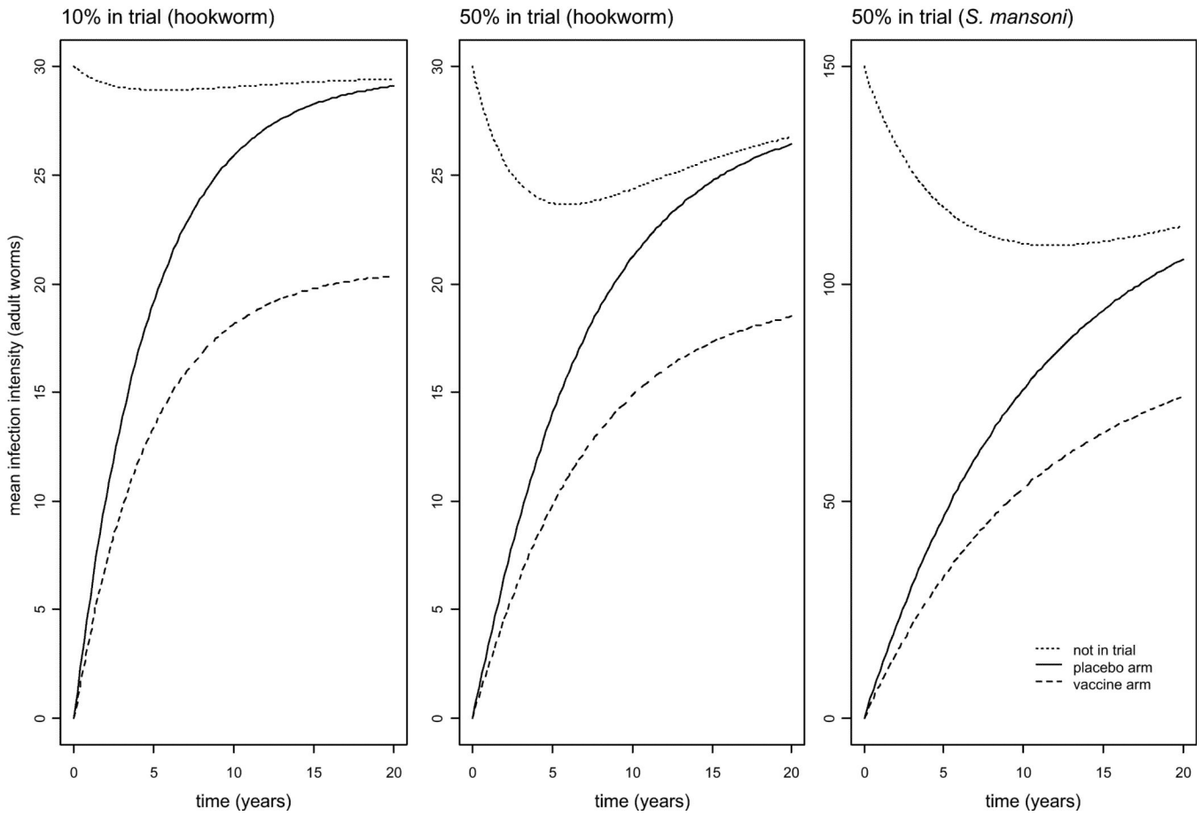
Fig. 4. Examples of model predictions of the change in mean parasite intensity over time. People in the trial, whether in the vaccine or placebo arm, are assumed to have any initial infections cleared at baseline.
