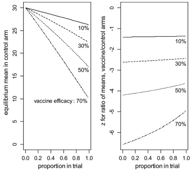
Fig. 5. The effect of vaccine efficacy and proportion of population in the trial on (a) the post-trial equilibrium mean in the control arm (left panel) and (b) Z statistic for the ratio of mean parasite intensity in vaccine/control arms (right panel).
